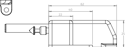
SCHLIESSBLECH C
